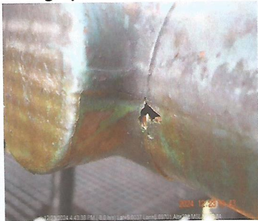
Fig.1: 7mm tear on the beam box
